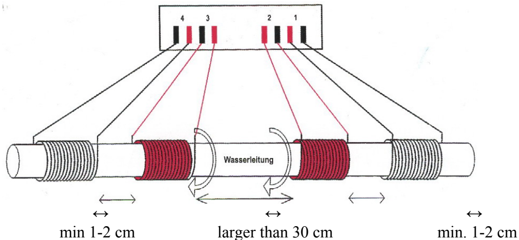
Typical mounting arrangement Showing wire connections on bottom of box
