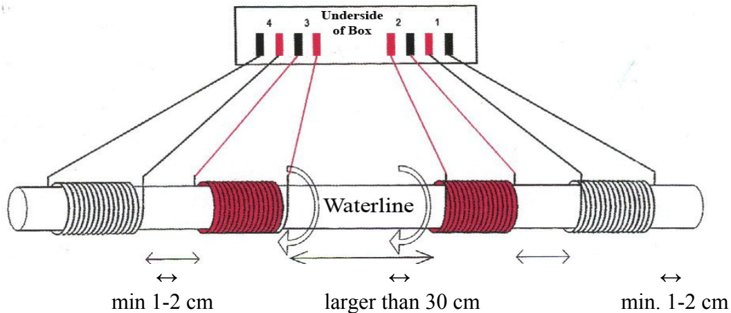
Typical mounting arrangement Showing wire connections on bottom of box
